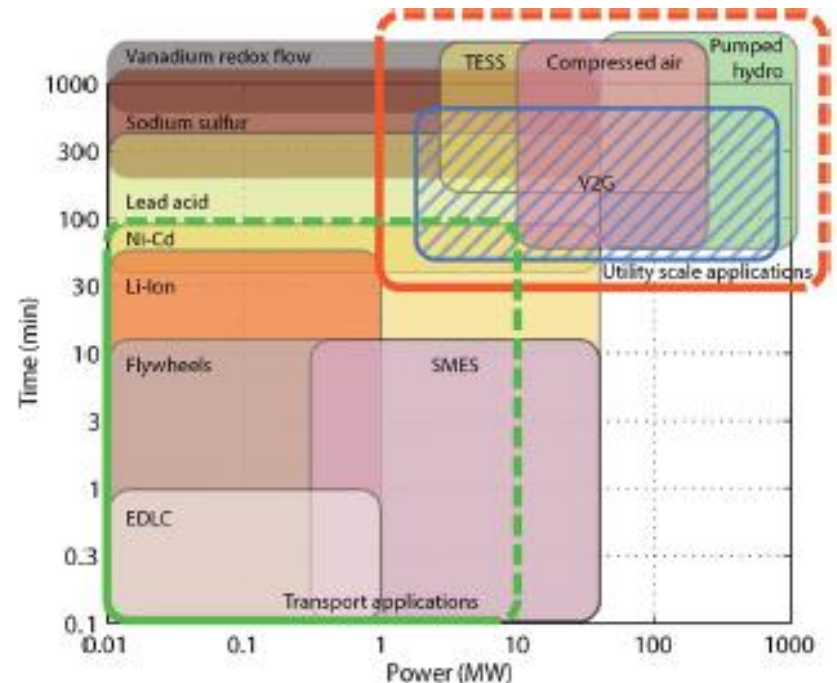
Storage technology discharge time vs. rated power
