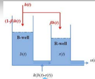
Kinetic Battery Model
