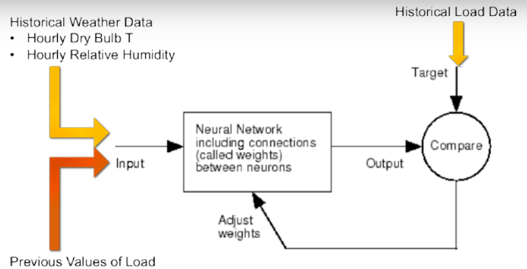
Nonlinear Autoregressive with Exogenous (NARX) Model
